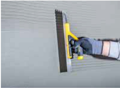
Figure 1 After adhering İstanbul Mavi thermal insulation boards and applying wall plugs, two layers of surface plaster is applied. İstanbul Mavi Plaster Mortar prepared is applied homogenously on the surface with a steel trowel.
