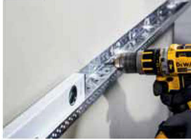
Figure 2 After the leveling process, İstanbul Mavi Socle Profiles are mounted using wall plugs.
