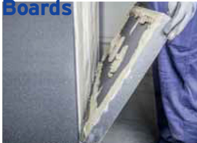
Figure 1 The thermal insulation board with adhesive mortar applied to its back should be placed onto the socle profile without any gaps.
